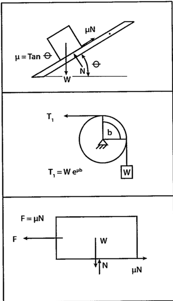
FIG. 3 Formulas for Calculation of Friction Coefficients, \mu F = Friction force, w = mass, N = Normal force b = angle of wrap (radians)
