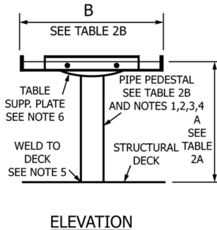
NOTE 1—See Notes 1 through 7 under Fig. 1. FIG. 2 Square Mess Table (Type II)
