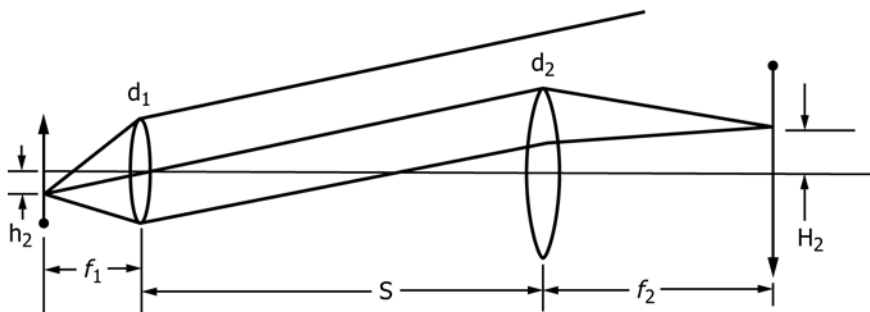
FIG. X4.2 Projector-Receiver Ray Trace for 50 % Vignetting Due to Lens L_2 Diameter d_2
