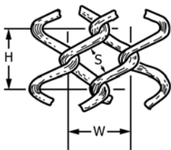
FIG. 1 Mesh Dimensions for ⅝-in., ½-in., and ¾-in. Fabric
