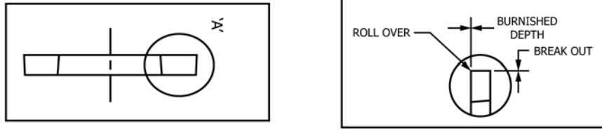
FIG. 1 Washer Inside Profile
