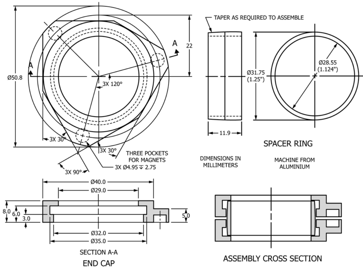
FIG. X1.1 Specimen Holder
