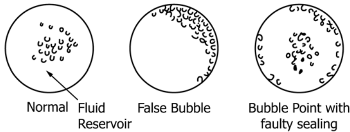
FIG. 5 Examples of Erroneous Bubble Points
