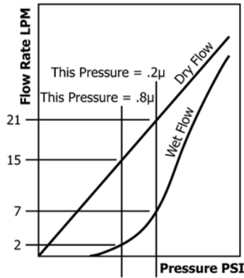
FIG. 9 Example of Pore Size Frequency Determination FIG. 9 Example of Pore Size Frequency Determination
