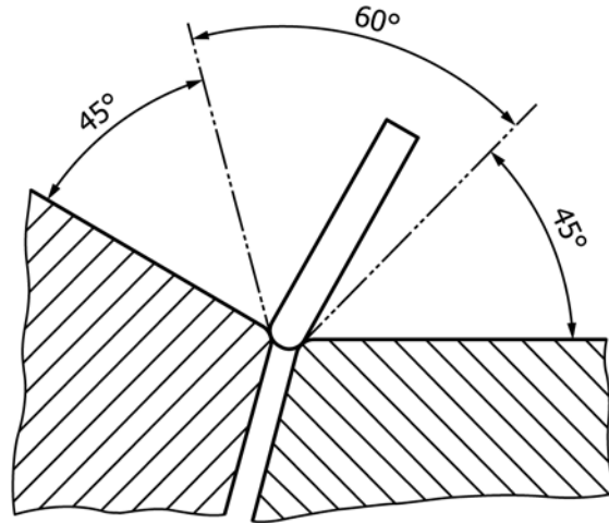
FIG. A1.18 Movement of Finger Probe—Reference 7.8.2.1
