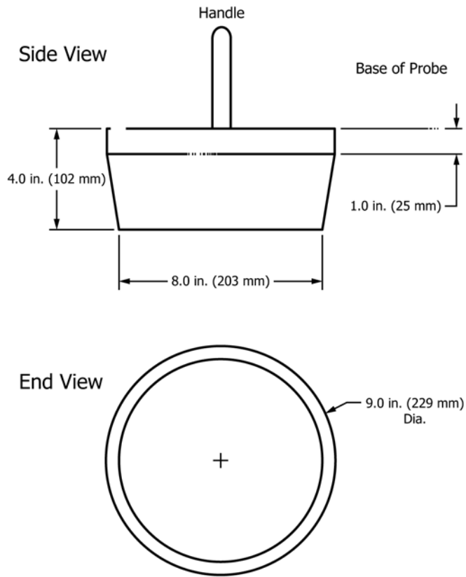
FIG. A1.3 Head Probe—Reference 7.8.6.2 and 7.8.6.3
