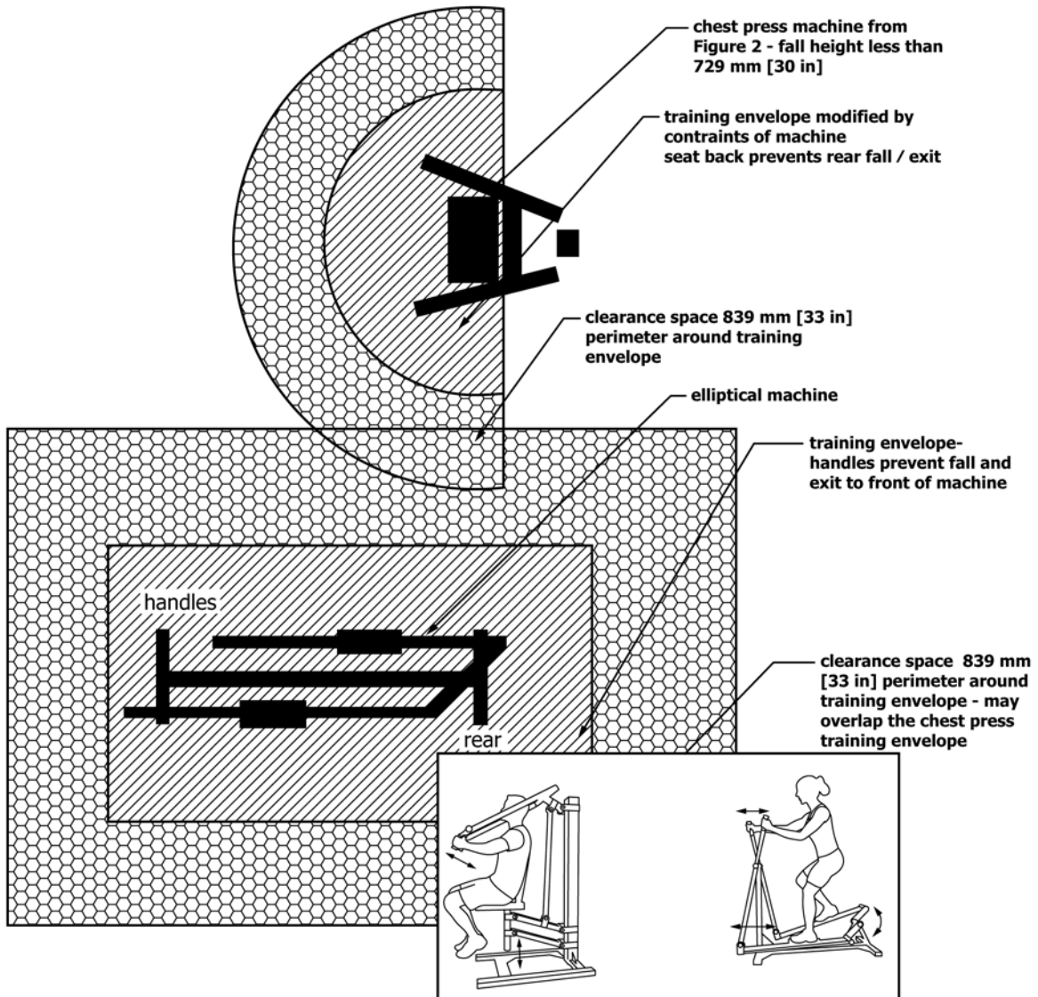
FIG. 6 Machine Layout
