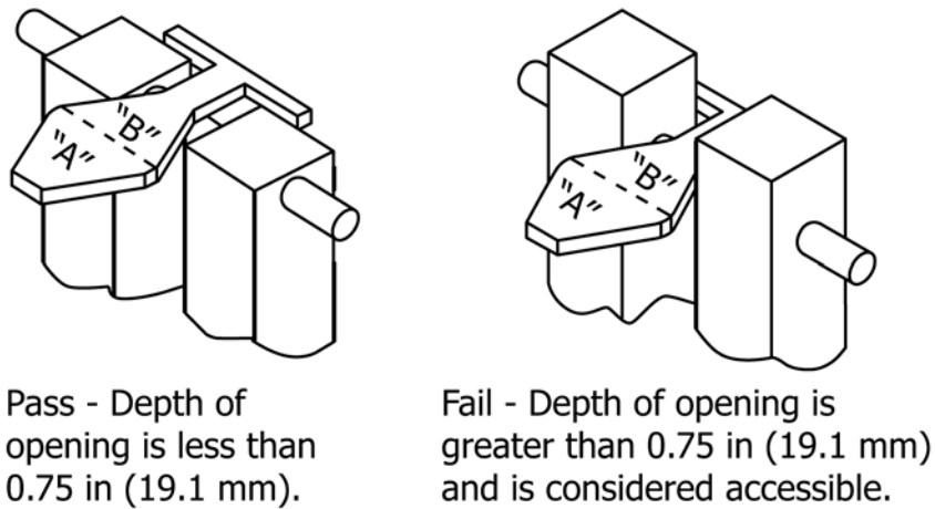
FIG. A1.9 A Partially Bounded Opening Is Not Considered Accessible if the Template Cannot Penetrate the Opening to a Depth Greater than 0.75 in. (19.1 mm) Thickness of the Test Template—Reference 7.8.6.3(4)
