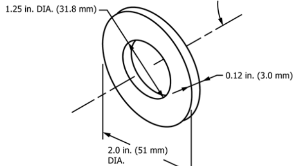
FIG. A1.11 Projection Test Gauge—Reference 7.7.1.1
