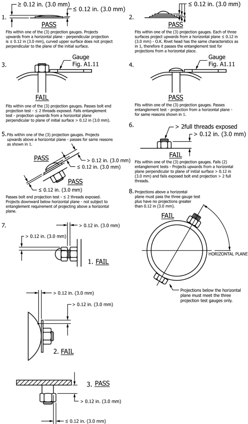
FIG. A1.16 Entanglement Test Requirement Examples—Reference 7.7.3
