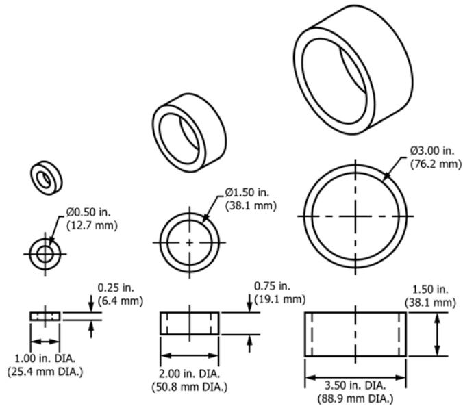
FIG. A1.10 Projection Test Gauges—Reference 7.6
