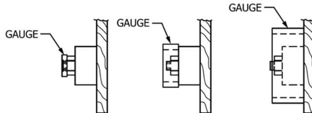
FIG. A1.12 Compound Projection Test—Reference 7.6.3
