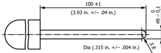
FIG. A1.17 Finger Probe—Reference 7.8.2.1
