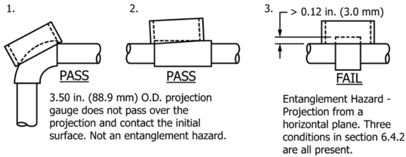
FIG. A1.14 Entanglement Test Requirement Examples—Reference 7.7.2
