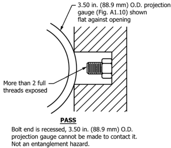
FIG. A1.15 Entanglement Test Requirement Examples—Reference 7.7.3
