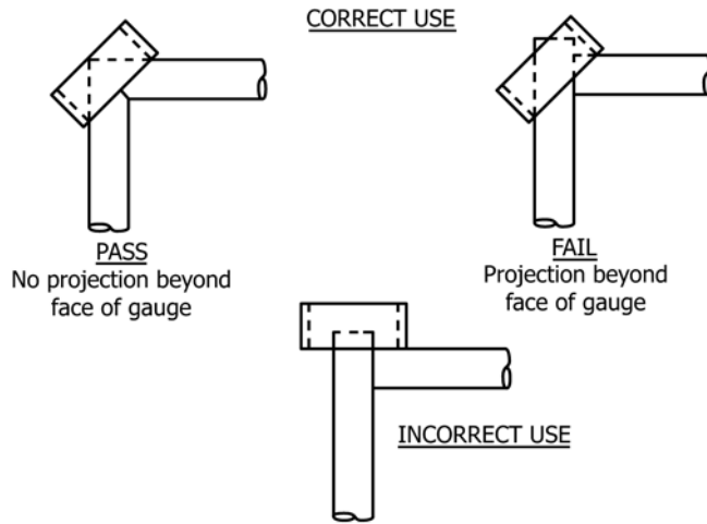
FIG. A1.13 Use of Projection Gauges—Reference 7.6.3
