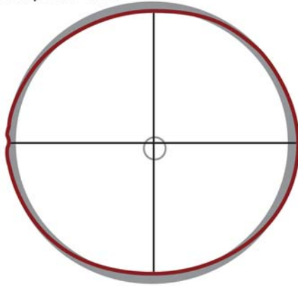
FIG. 2 Single Point Image of Uneven Deformation of Pipe
