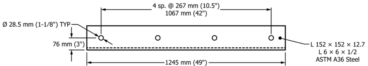
FIG. A2.2 Details for Surrogate Test Vehicle Impactor Nose
