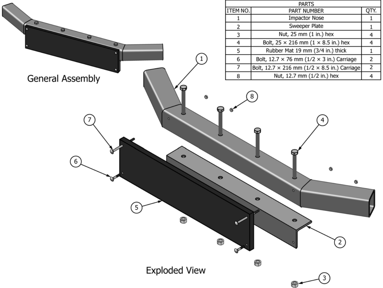
FIG. A2.1 Surrogate Test Vehicle Impactor Nose
