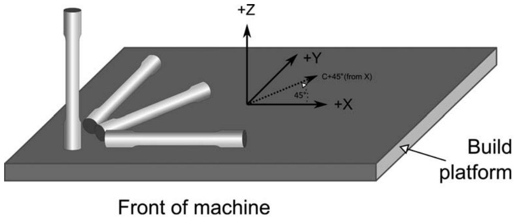
FIG. X2.1 Build Platform
