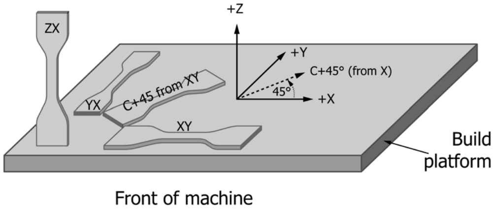
FIG. X1.1 Build Platform
