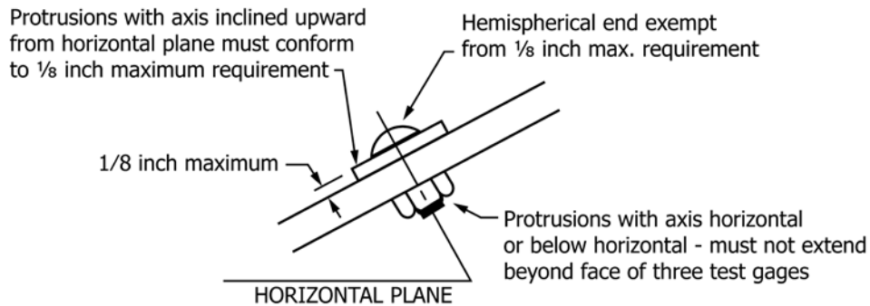
FIG. 11 Upright Protrusion Test
