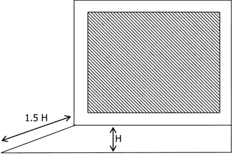
FIG. 15 Tread Depth of Step and Ramp
