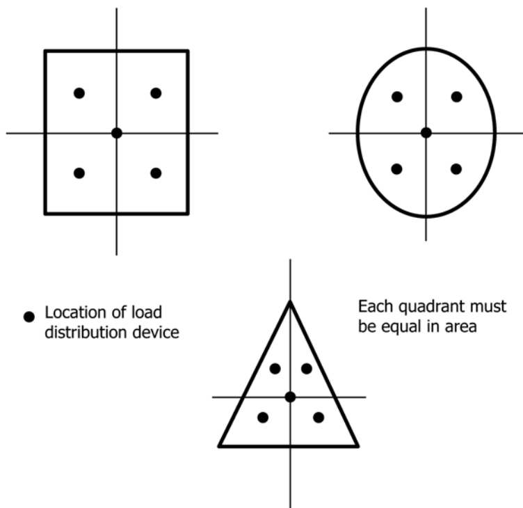
FIG. 2 Example of Test Position Grid
