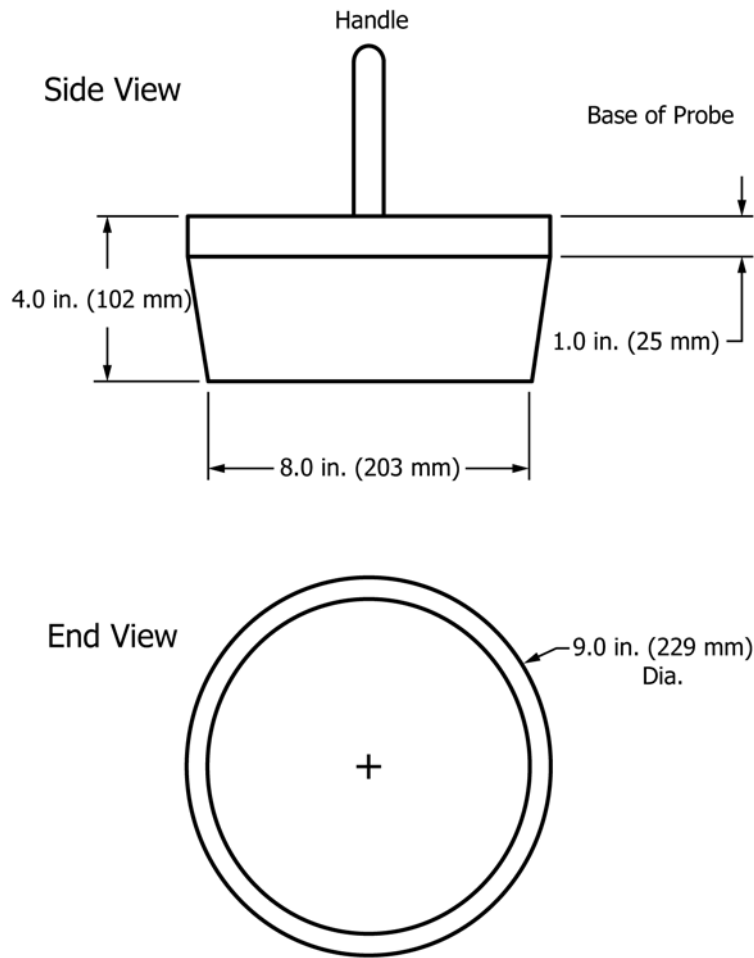
FIG. 4 Head Probe
