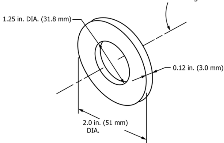
FIG. 9 Additional Protrusion Gauge
