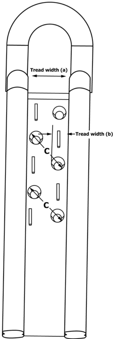
FIG. 16 Rung Distance Measurements
