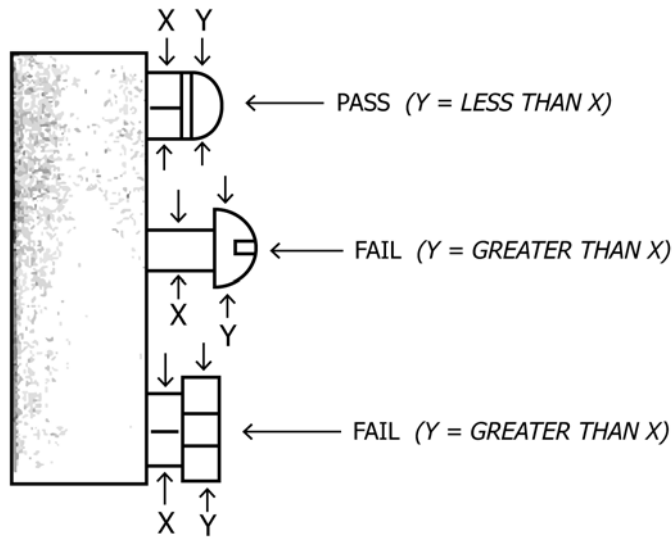
FIG. 13 Examples of Protrusion Configuration
