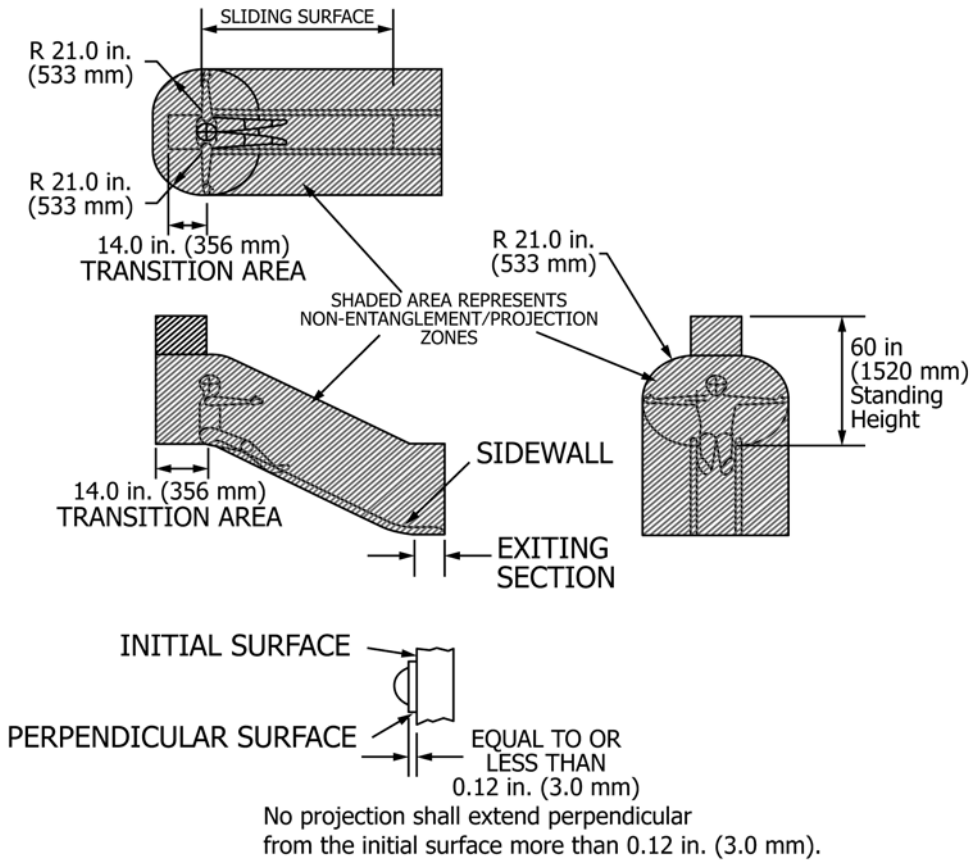
FIG. 12 Areas Subjected to 6.7.6.1
