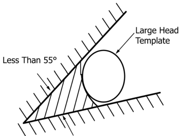
FIG. 6 In-Fill Shield for Angles Less than 55°
