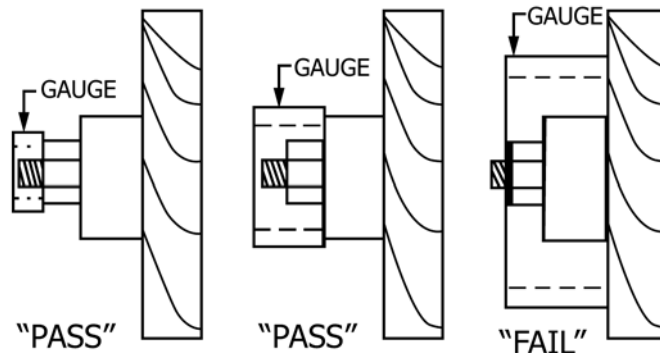
FIG. 10 Compound Projection Test
