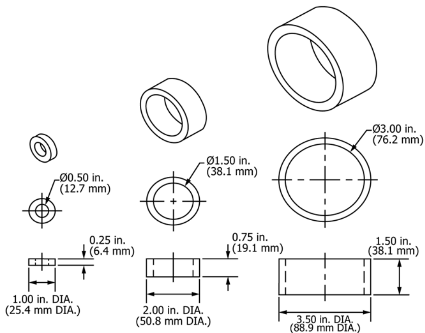
FIG. 8 Protrusion Gauges
