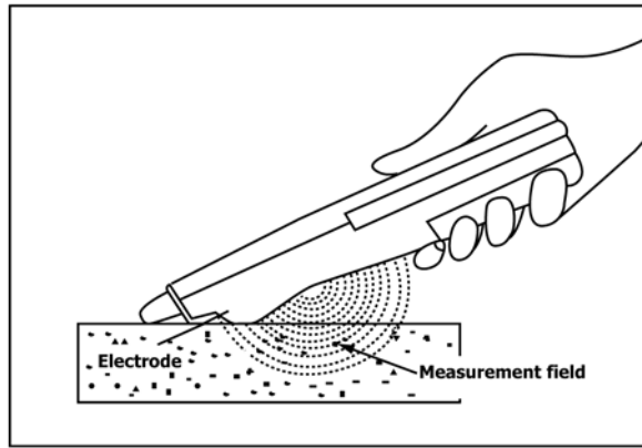
FIG. X2.2 Moisture Meter for Concrete and Other Floor Slabs with Different Electrodes and Positioning on Surface of the Floor Slab.
