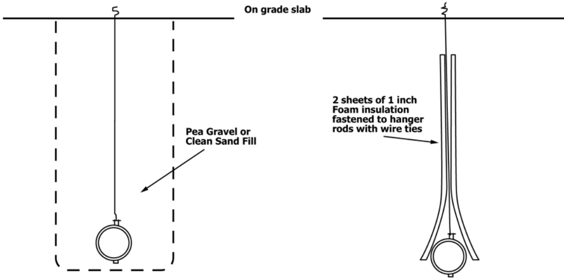
FIG. 1 Load Limiting Methods
