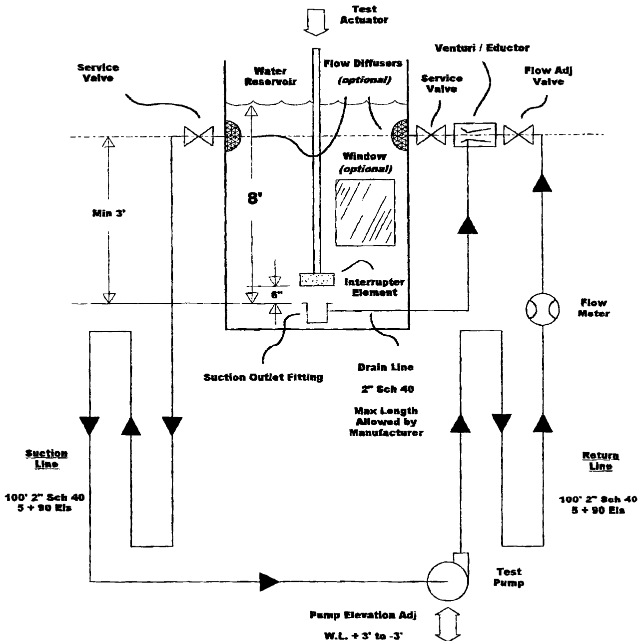
FIG. 3 Safety Vacuum Release System (SVRS) Vacuum-Induced, Indirect Drain System
