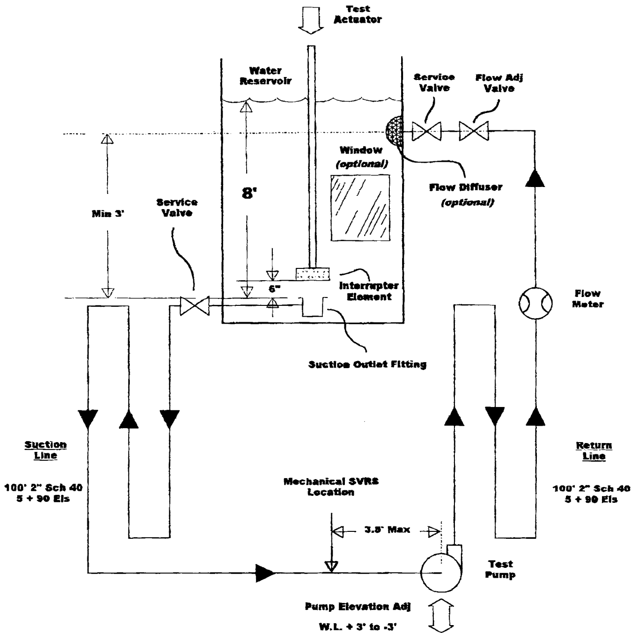
FIG. 2 Safety Vacuum Release System (SVRS)
