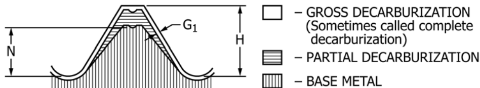
FIG. 1 Decarburization Zones
