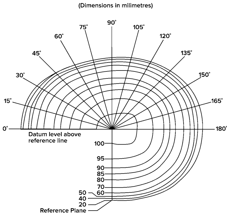
FIG. A1.2 Horizontal Half-Sections at Datum Levels
