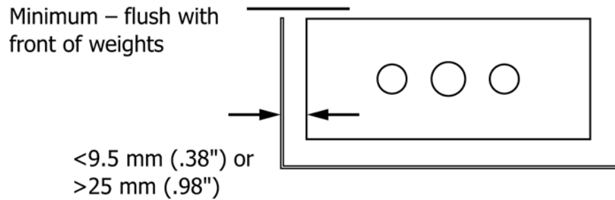
FIG. 9 Weight Enclosure Spacing
