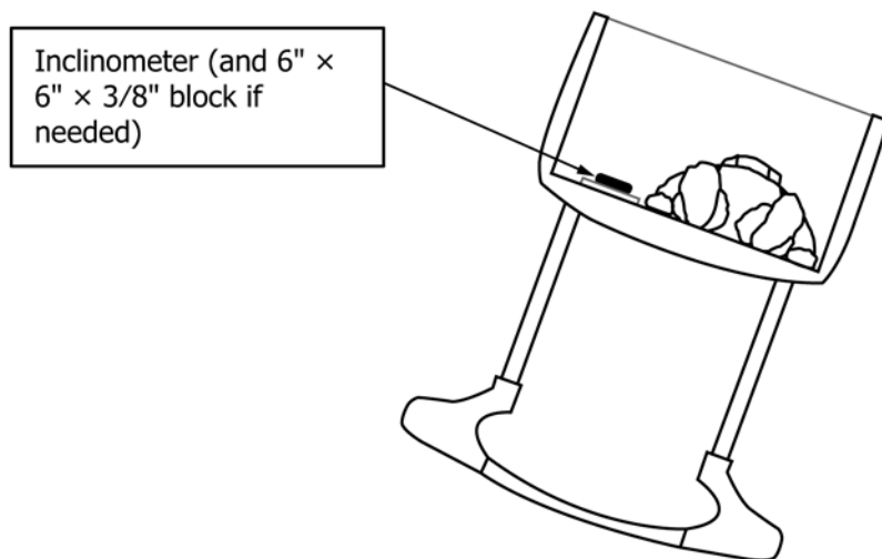
FIG. 22 Maximum Side-to-Side Rock/Swing Angle
