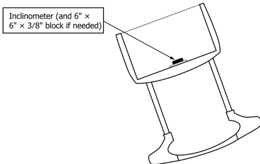
FIG. 20 Maximum Deflection Angle
