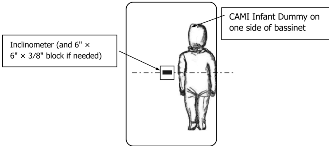
FIG. 21 Placement of Inclinometer and CAMI Infant Dummy
