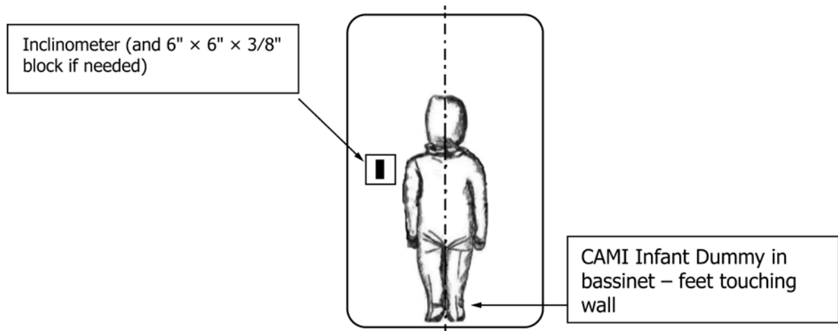
FIG. 25 Placement of Inclinometer and CAMI Infant Dummy
