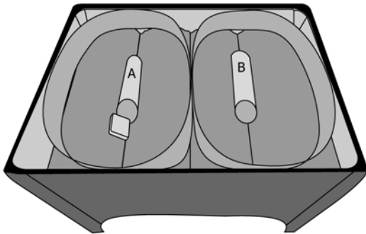
FIG. 15 Steel block in Front of Cylinder for 2-Occupant Bassinet
