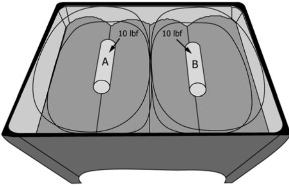
FIG. 14 Placement of Cylinders for 2-Occupant Bassinet
