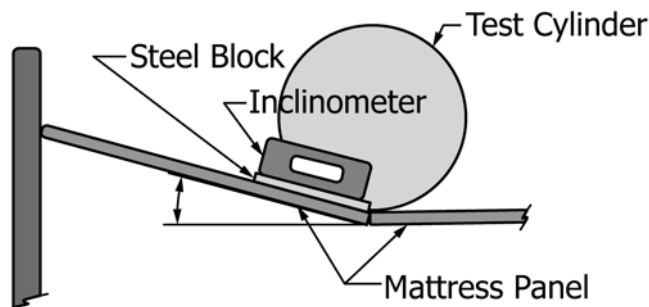
FIG. 12 Inclinometer on Steel Block in Front of Cylinder for a Single-Occupant Bassinet
