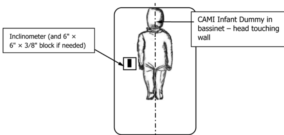
FIG. 24 Placement of Inclinometer and CAMI Infant Dummy
