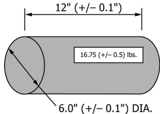
FIG. 9 Infant Test Cylinder
