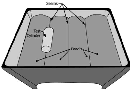
FIG. 10 Cylinder Placement on Mattress Seam
