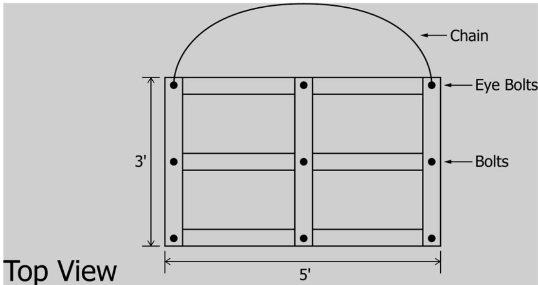
FIG. X2.1 Nail Drag Diagram
