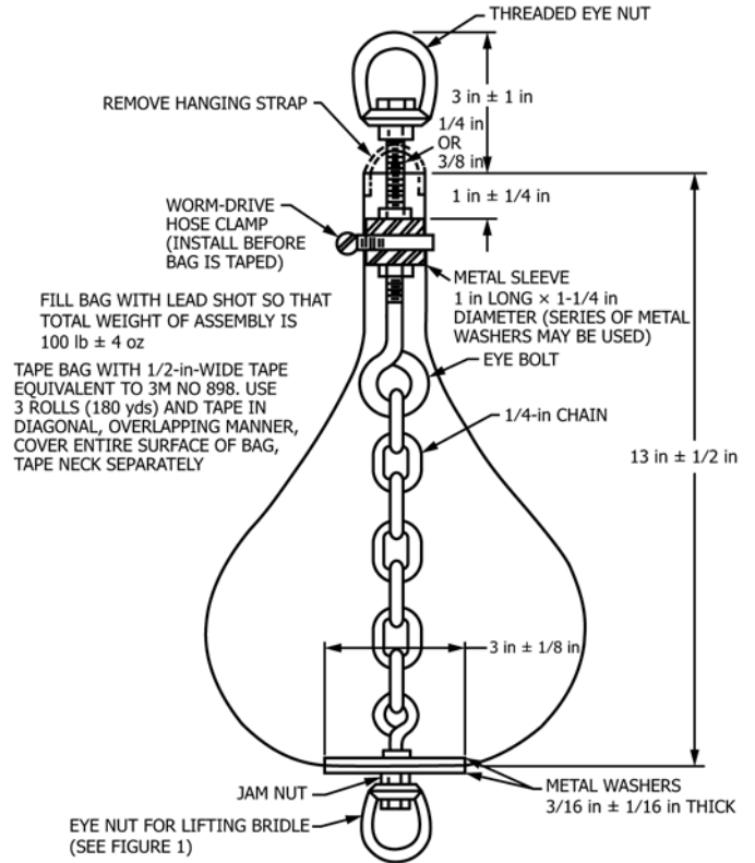
Figure 3 Impactor
