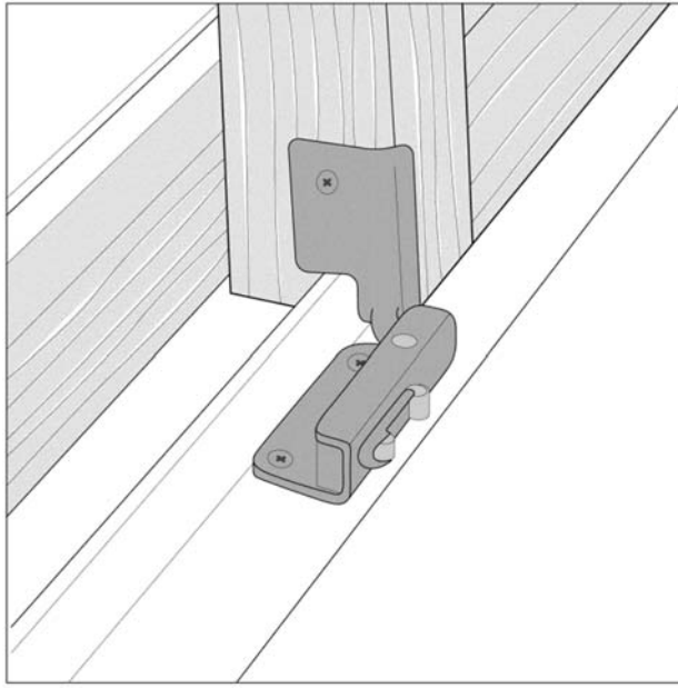
FIG. X5.5 Sample Gliding Window Style Window Opening Control Device
