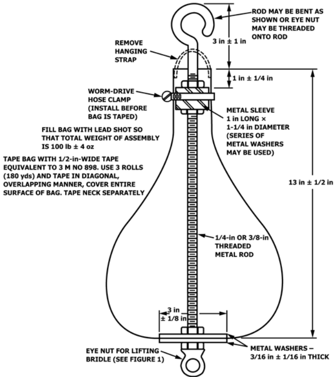
Figure 2 Impactor
