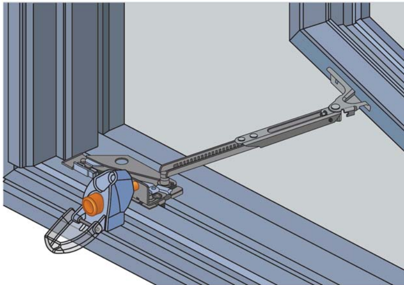
FIG. X5.2 Sample Casement Style Window Opening Control Device
