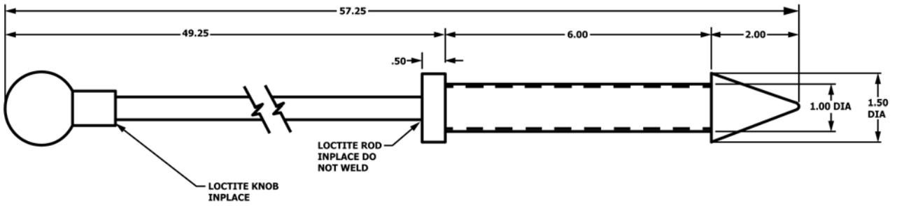
NOTE 1—All dimensions are in inches. FIG. A1.1 Magnetic Test Probe
