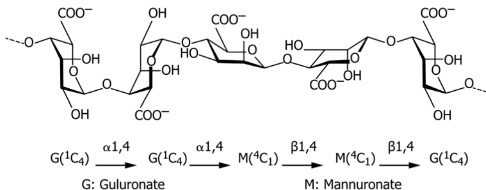
FIG. X2.1 Alginate Chain
