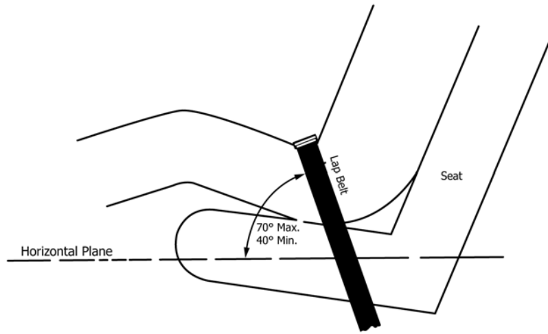
FIG. 1 Proper Lap Belt Mounting Angle
