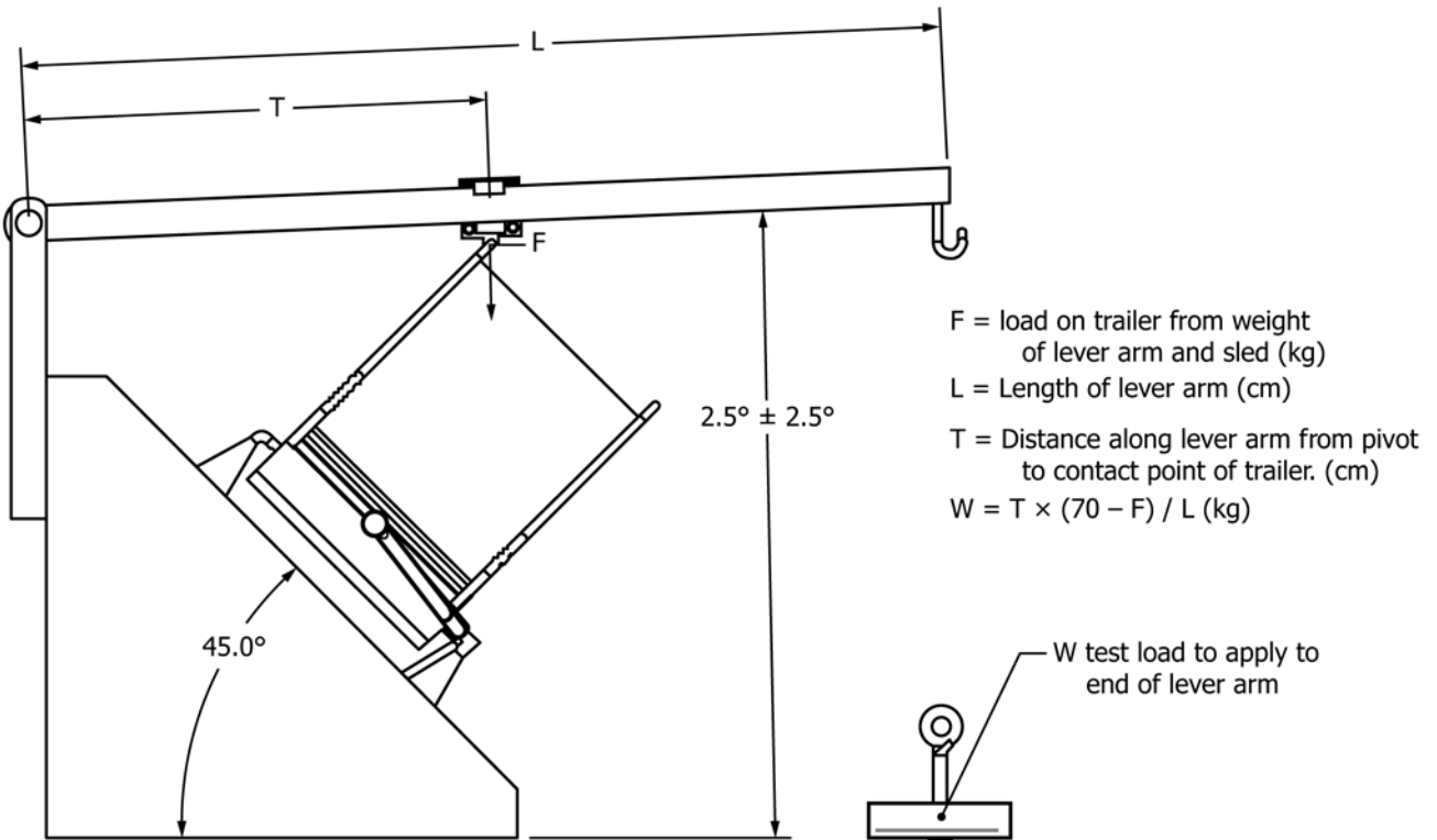
FIG. 2 Roll Test Before Load is Applied
