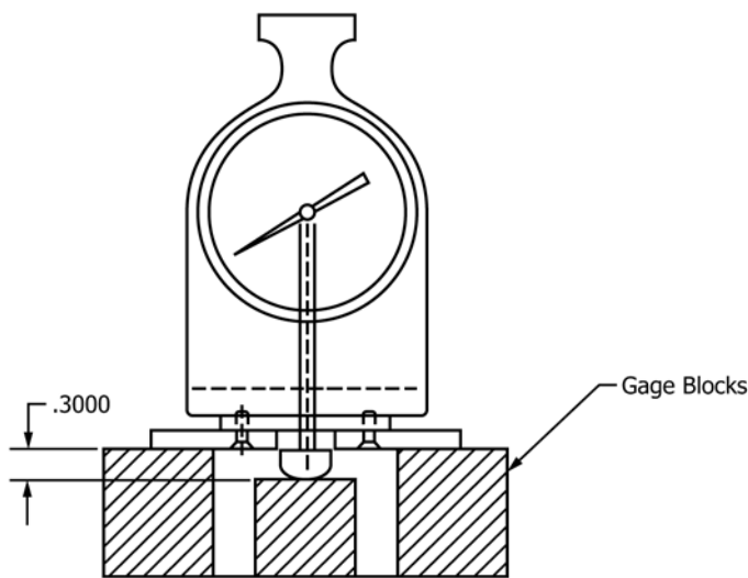
Gage Block Setup for "0" Reading
