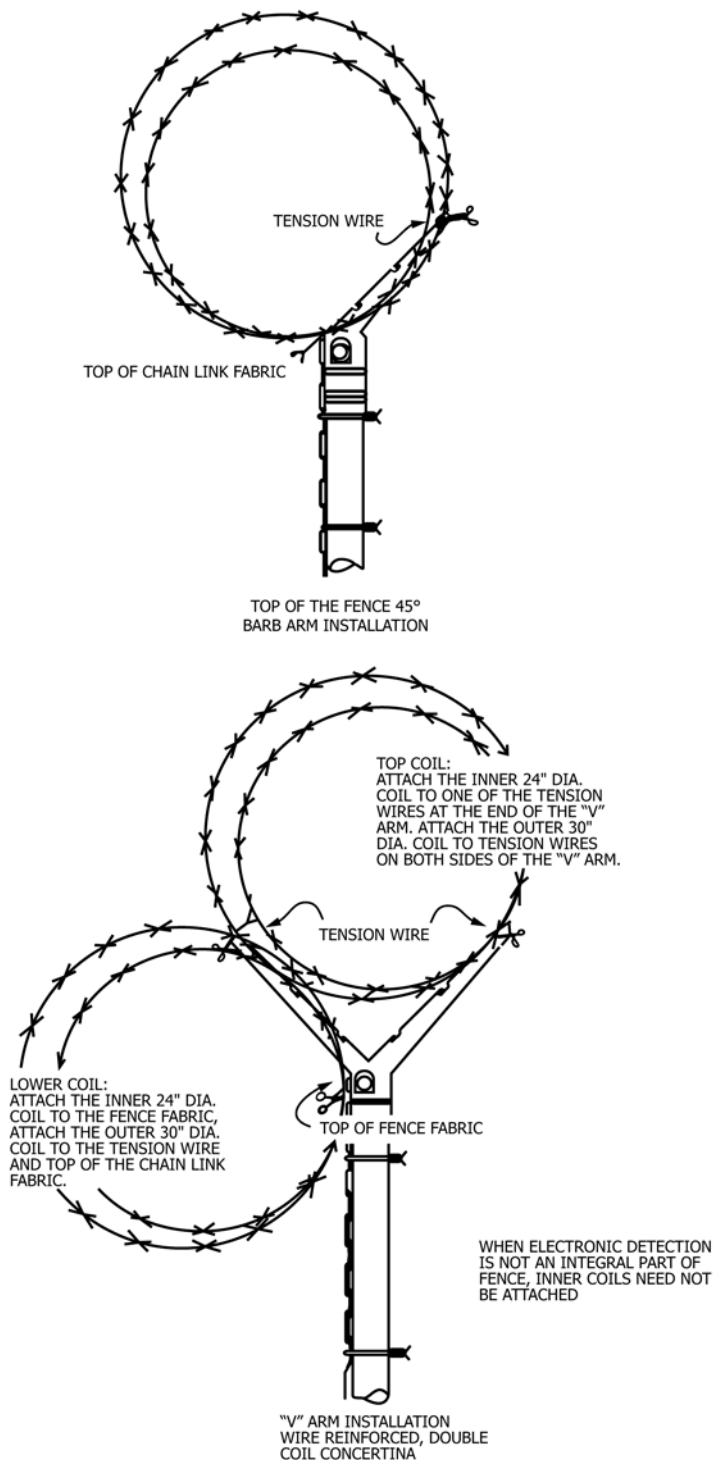
FIG. 8 Wire Reinforced Double Coil Concertina
