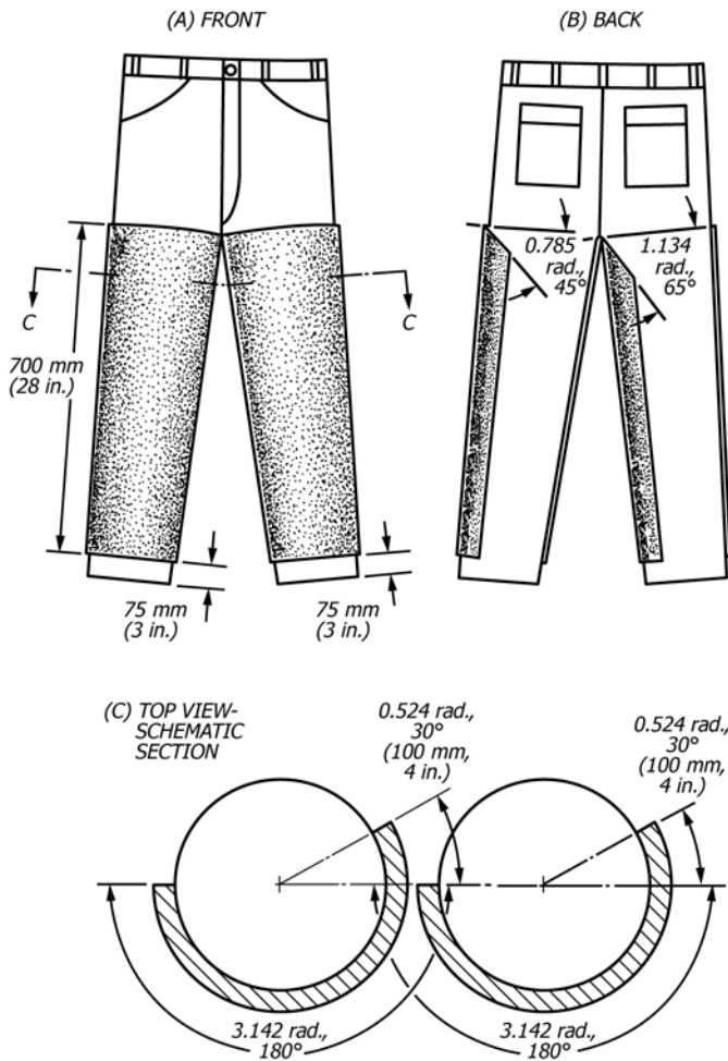
FIG. 1 Protective Pants / Trousers
