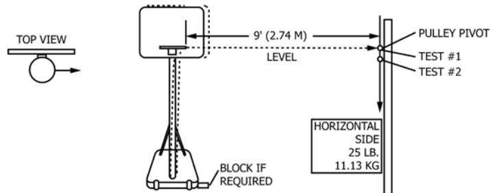
FIG. 6 Portable Base Horizontal Side Testing
