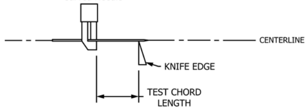
Knife Edge Bend Test Curved Needle
