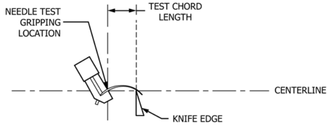
Knife Edge Bend Test Curved Needle
