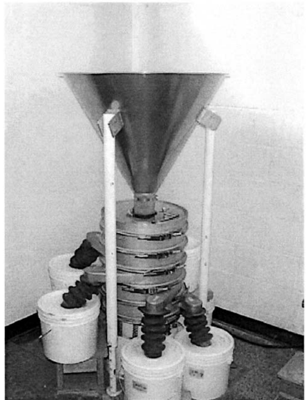
FIG. 9 Continuous Flow Vibrating Sieve
