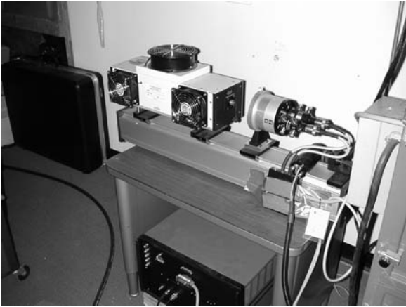
FIG. 6 Laser Doppler Power Supply and Instrumentation
