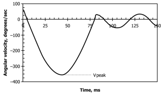
FIG. 4 First Derivative of the Rearfoot Angle Time History Shown in Fig. 3
