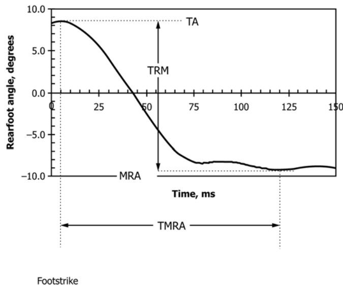
FIG. 3 Typical Time History of the Rearfoot Angle During a Running Step
