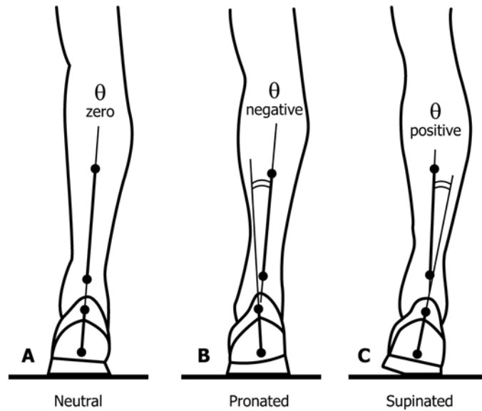
FIG. 2 Posterior View of the Right Foot and Lower Leg Showing the Rearfoot Angle, \theta , Defined as the Angle Between the Transverse Vertical Plane Projection of the Line Formed by the Leg Markers and the Transverse Vertical Plane Projection of the Line Formed by the Specimen Markers
