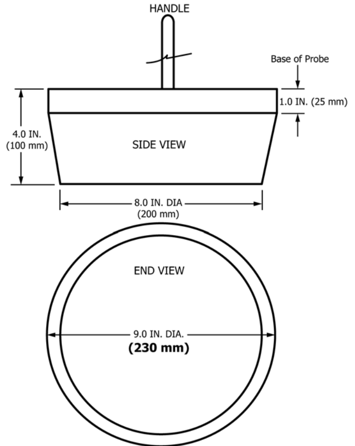
FIG. 9 Head Probe
