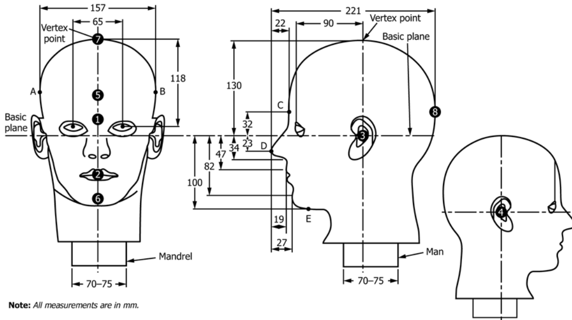
FIG. 6 Headform Details to Determine Coverage Level of EHPD
