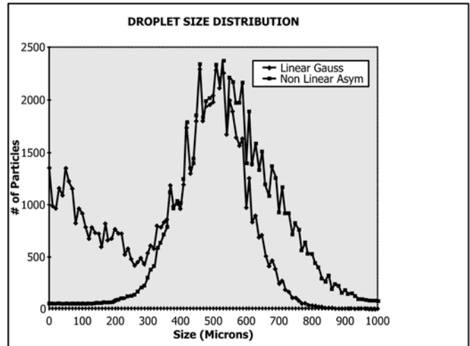
FIG. 2 Droplet Size Distribution
