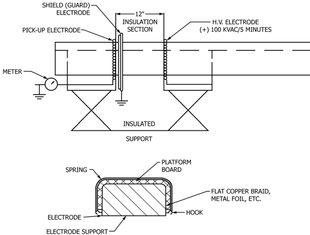
FIG. 2 Insulating Segment of Platform
