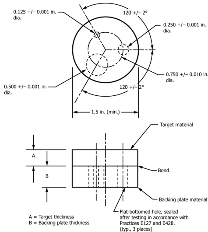
FIG. 1 Reference Block
