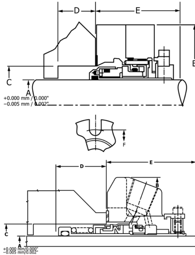
Maximum Dimensions for Seal Installation
