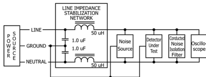
FIG. 3 Configuration for the Low-Level Conducted Noise Test
