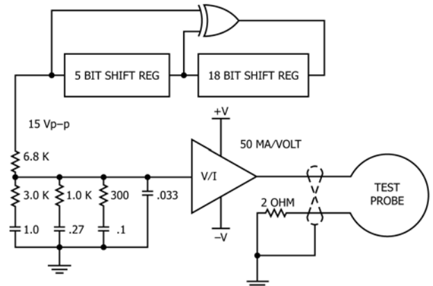
FIG. 6 Suggested Approach for the Audio Frequency Noise Test
