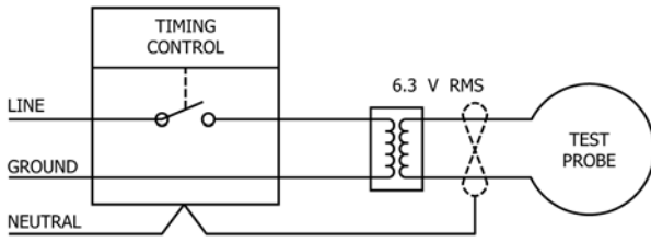
FIG. 4 Suggested Approach for the Transient Hum Test
