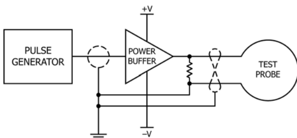
FIG. 5 Suggested Approach for the Noise Spike Test
