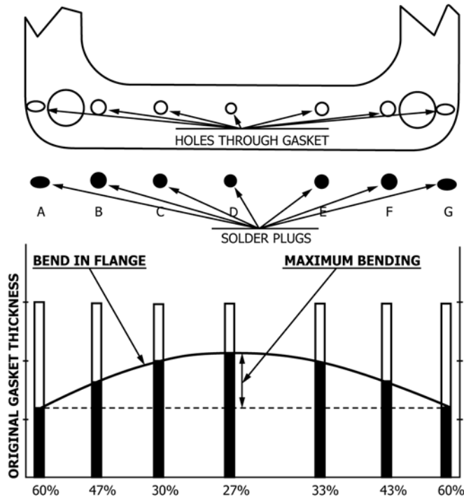
FIG. 2 Suggested Plot of the Solder-Plug Test Data
