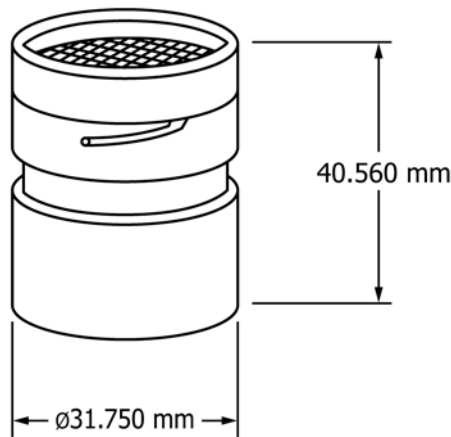
FIG. 1 Sample Cell
