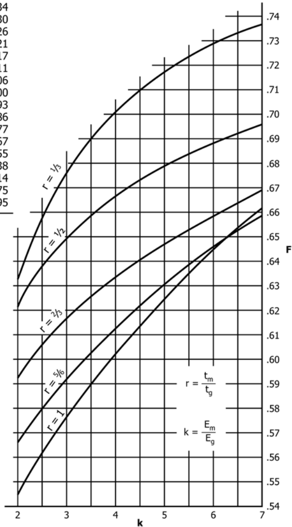
FIG. 4 Shape Modulus Factor, F, for Given Values of r, the Ratio of Thicknesses and k, the Ratio of Young's Moduli, for Determining the Expansion Mismatch in Disk-Seals
