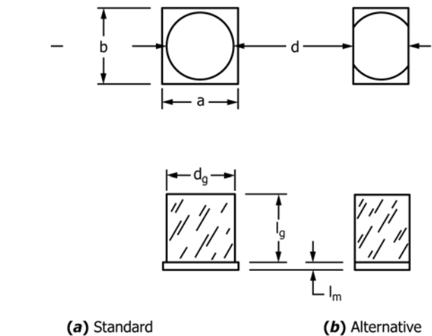
FIG. 2 Sheet Seals
