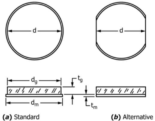
FIG. 3 Disk Seals
