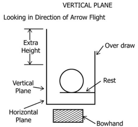
FIG. 4 Extended Height of the Vertical Plate
