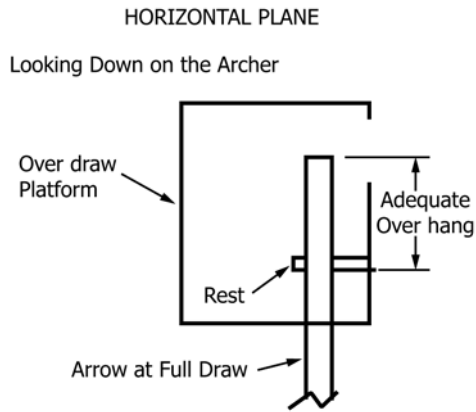
FIG. 6 Adequate Overhang of the Arrow Relative to the Rest
