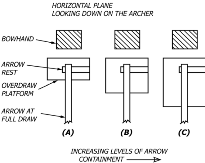
FIG. 2 Increasing Levels of Arrow Containment, Horizontal Plane
