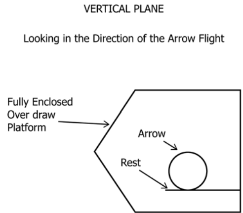
FIG. 5 Fully Enclosed Overdraw System
