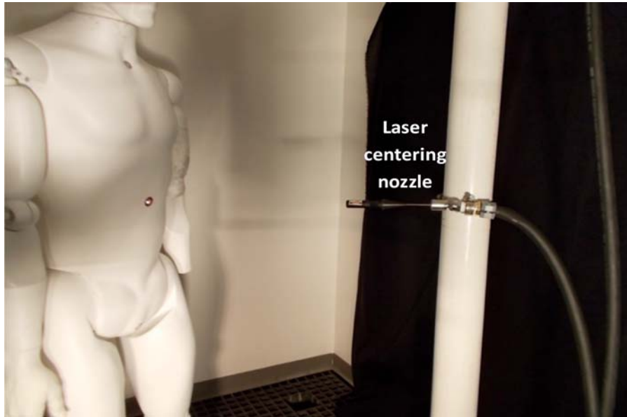
FIG. A1.7 Ensuring Correct Height of Middle Nozzle with Respect to Center Target on Manikin
