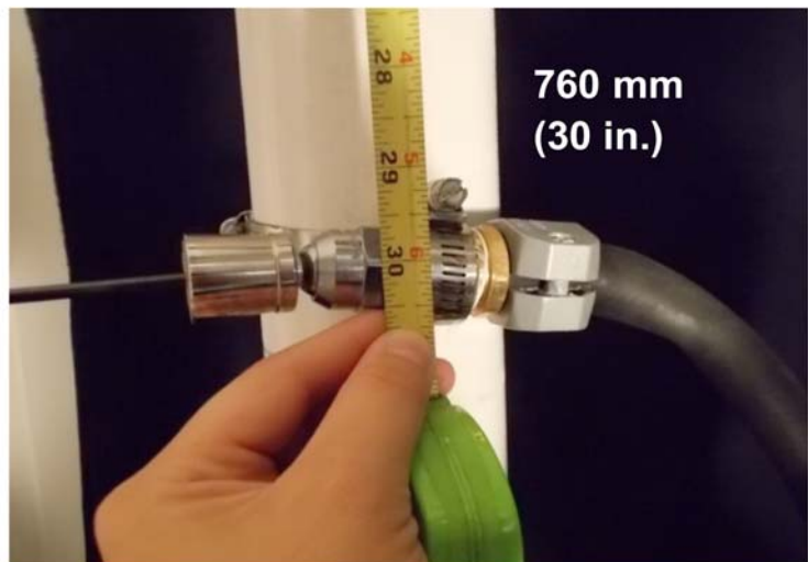
FIG. A1.9 Locating Height of Top Spray Nozzle with Respect to Middle Spray Nozzle
