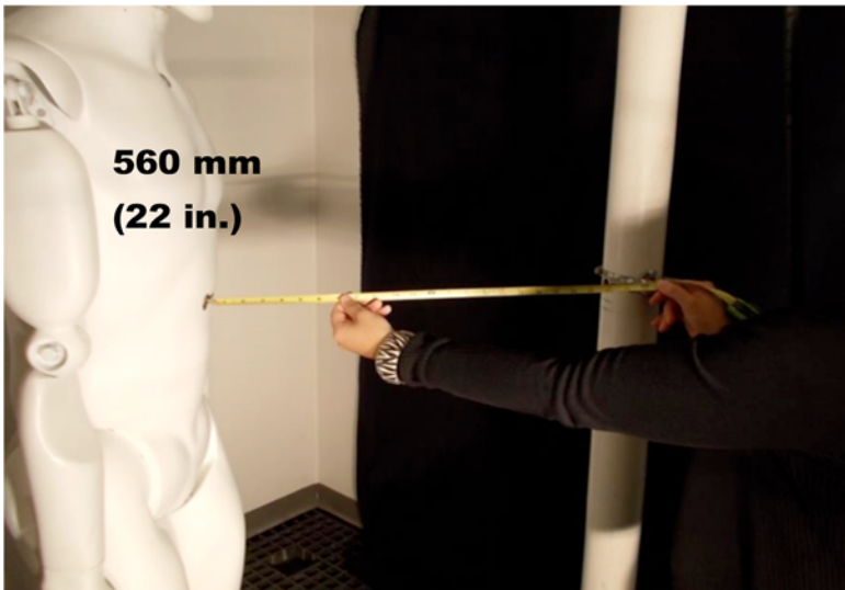
FIG. A1.5 Measuring Distance from Central Nozzle to Center Manikin Target
