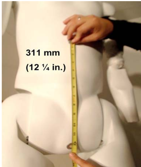
FIG. A1.4 Measurement to Position Bottom Manikin Target
