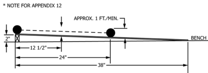
FIG. 1 Hard-Crease Fixture
