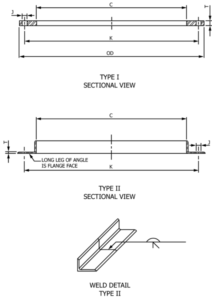
FIG. 1 Flanges, Types I and II
