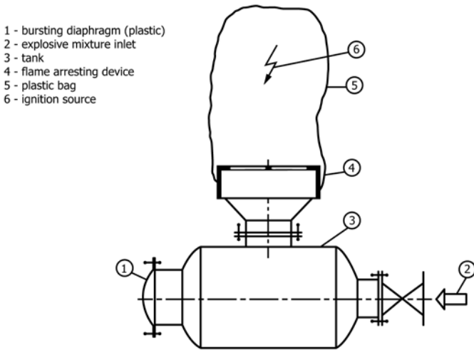
FIG. 1 Test Rig for Flash Back Test
