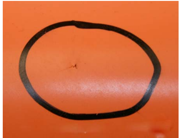
FIG. 5 Breakdown (Dielectric Failure Blanket: Front)
