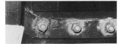
GALVANIC CORROSION/ COATING UNDERCUTTING
