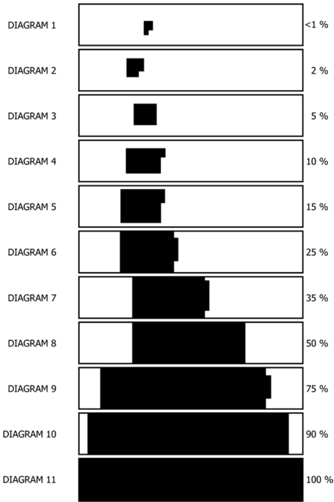
FIG. 1 Overall Extent of Failure Diagrams
