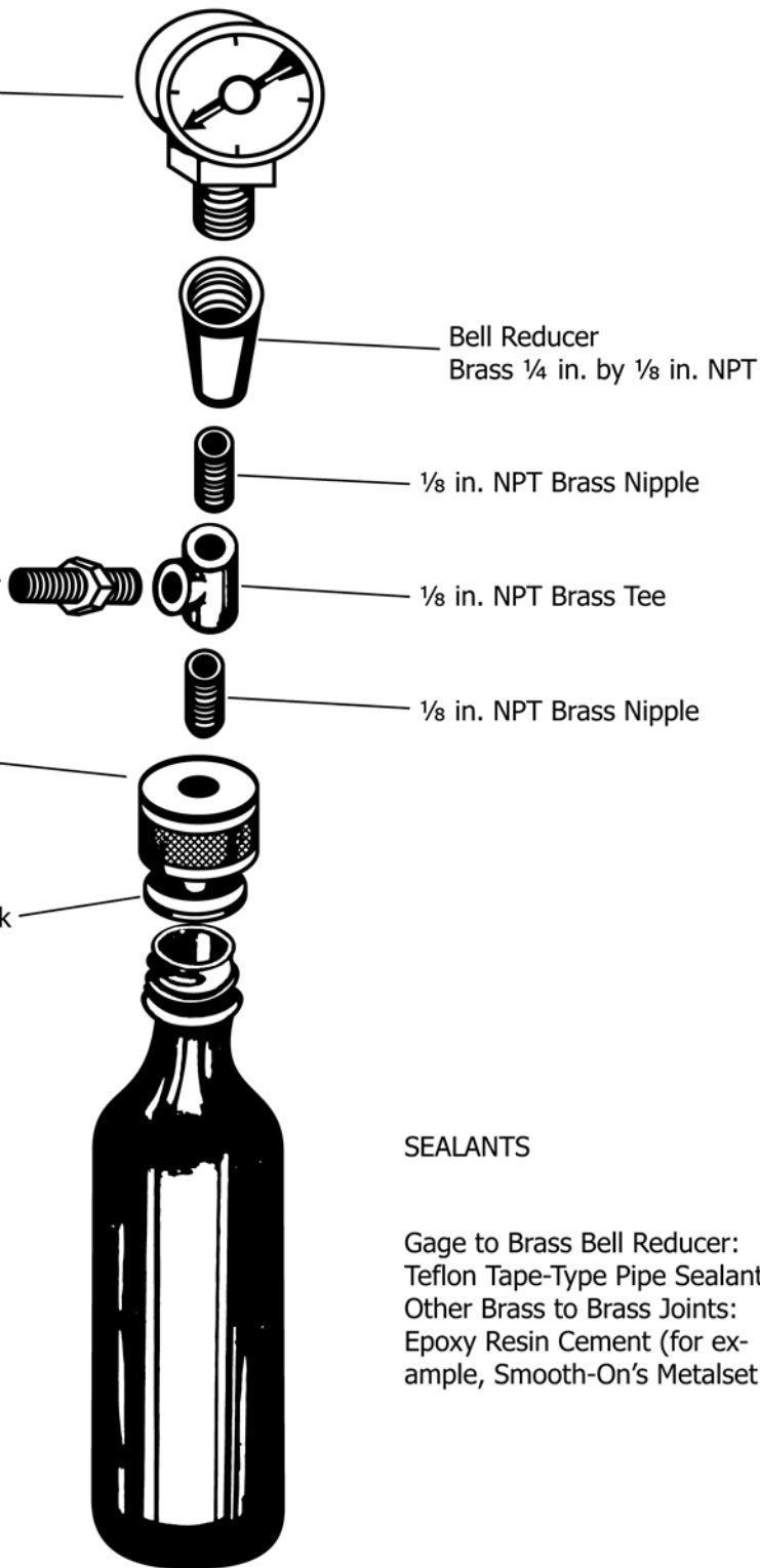
FIG. 3 Pressure Monitoring Assembly
